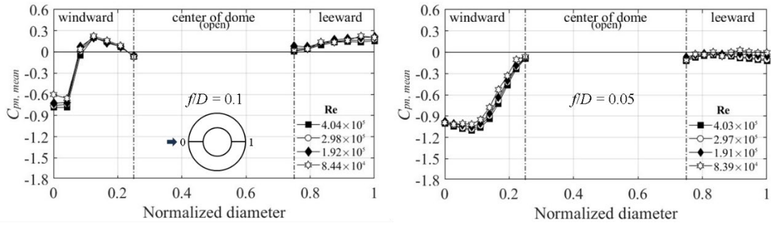
<Fig. 12> Mean net pressure coefficient according to Reynolds number in Uniform flow
