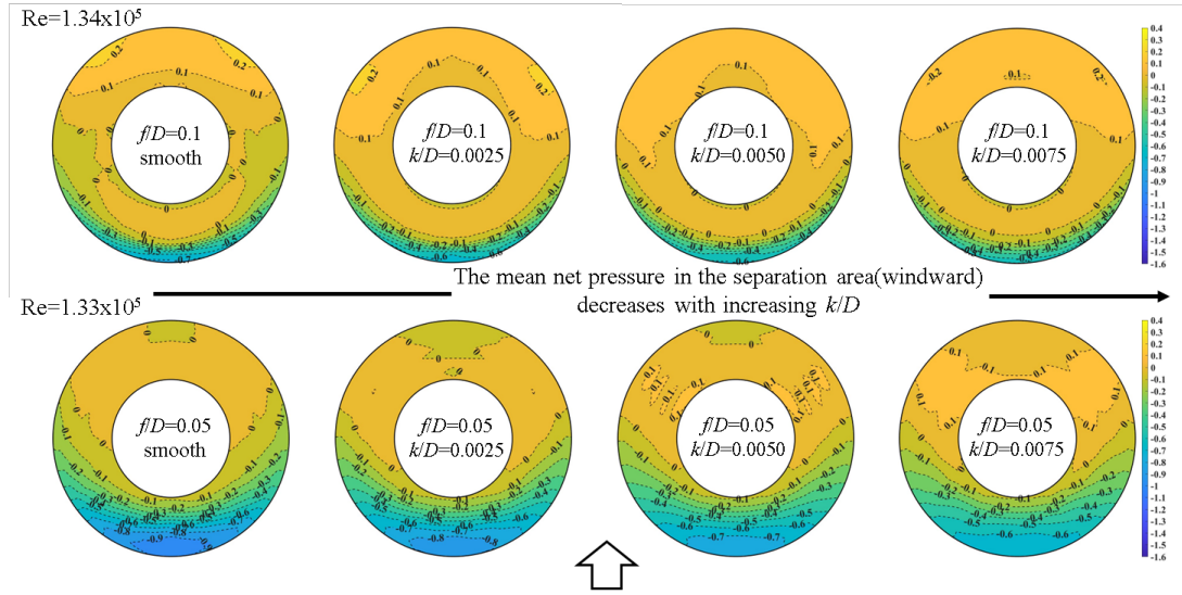
<Fig. 15> Distribution of mean net pressure coefficient according to k/D
