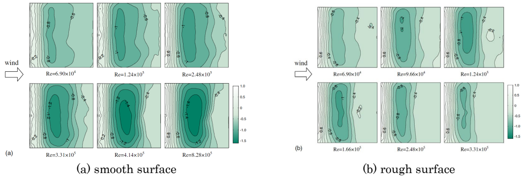
<Fig. 1> Contours of mean pressure distributions of cylindrical roofs at various Reynolds numbers (Qiu et.al (2018))
