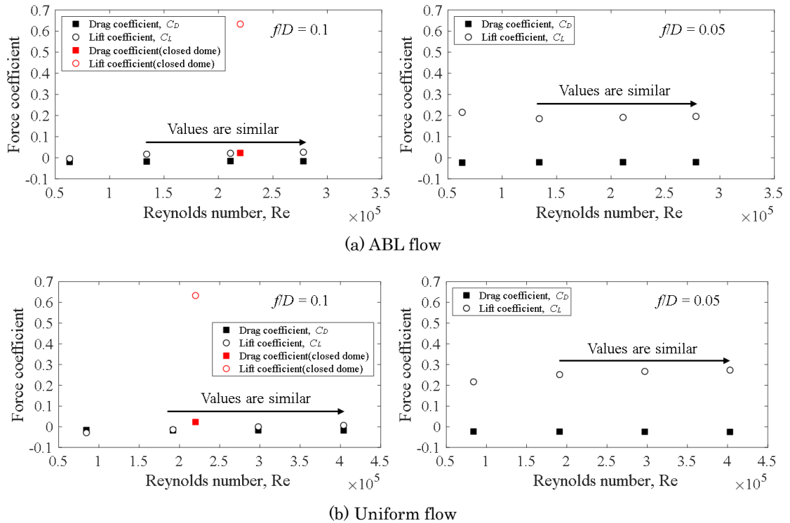
<Fig. 16> Drag and lift force coefficients
