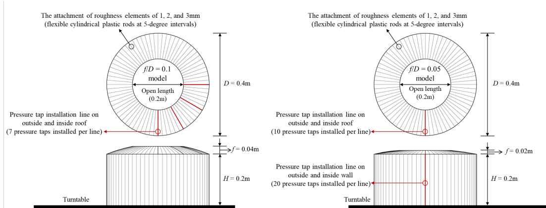
<Fig. 4> Dimensions of the model, pressure taps, and surface roughness elements
