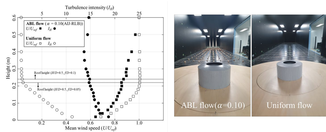
<Fig. 7> Characteristics of oncoming flow
