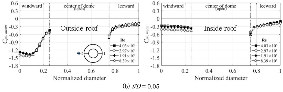
<Fig. 11> Mean pressure coefficient according to Reynolds number in Uniform flow
