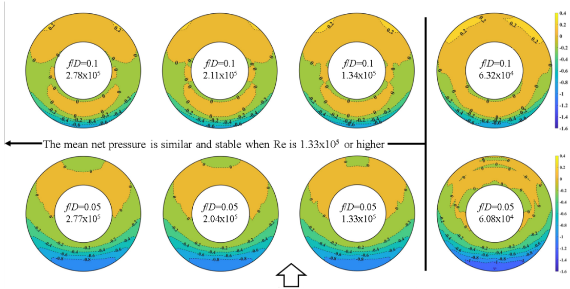
<Fig. 10> Distribution of mean net pressure coefficient according to Reynolds number in ABL flow
