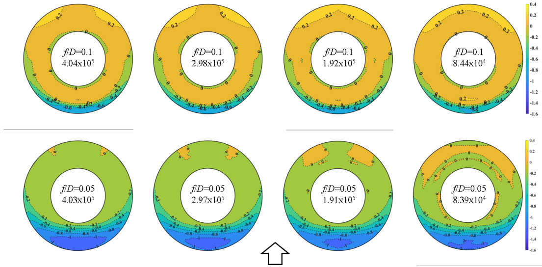
<Fig. 13> Distribution of mean net pressure coefficient according to Reynolds number in Uniform flow
