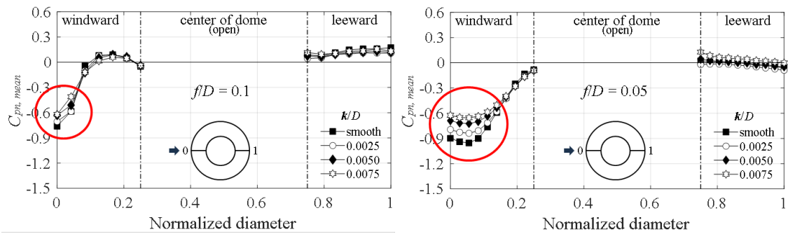
<Fig. 14> Mean net pressure coefficient according to k/D
