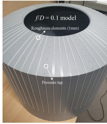
<Fig. 5> The roughness elements attached to the actual model
