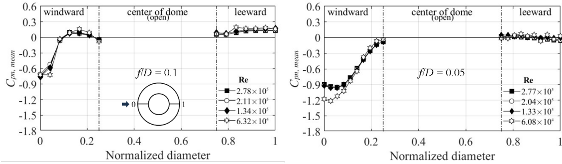
<Fig. 9> Mean net pressure coefficient according to Reynolds number in ABL flow
