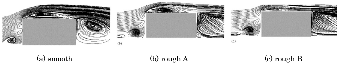
<Fig. 2> Streamlines of the mean flow projected onto the symmetry plane of the building
